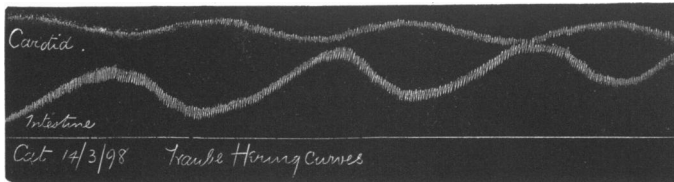
Fig. 1. Traube-Hering curves. \frac{1}{2} .
