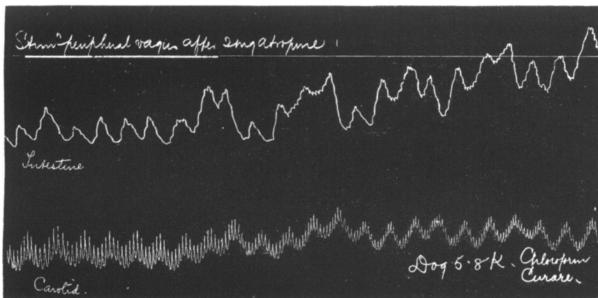
Fig. 15. Unusual effect obtained in one dog by excitation of the vagus. Dilatation of the intestinal vessels could not be made out by direct observation of the intestine. \frac{1}{2} .
